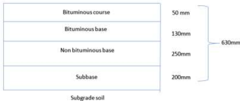
Fig -7: Pavement Thickness
