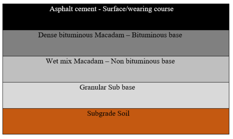
Fig -8: Pavement Design
