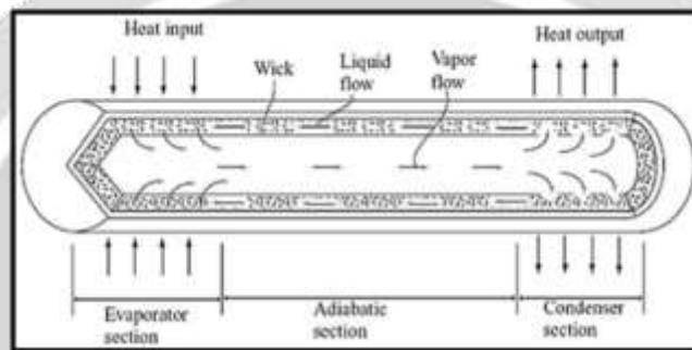
FIG: SCHEMATIC DIAGRAM OF NANOPIPE
