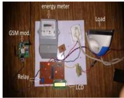
Fig -3: Experimental Setup
