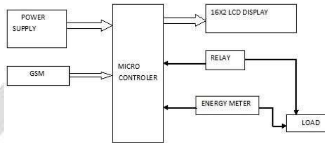
Fig -1: Block diagram of Prepaid Energy meter system
