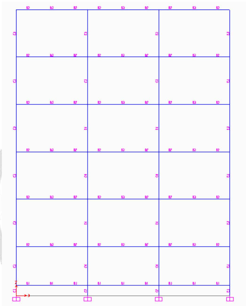
Fig : 4 Assigning the Member Sections
