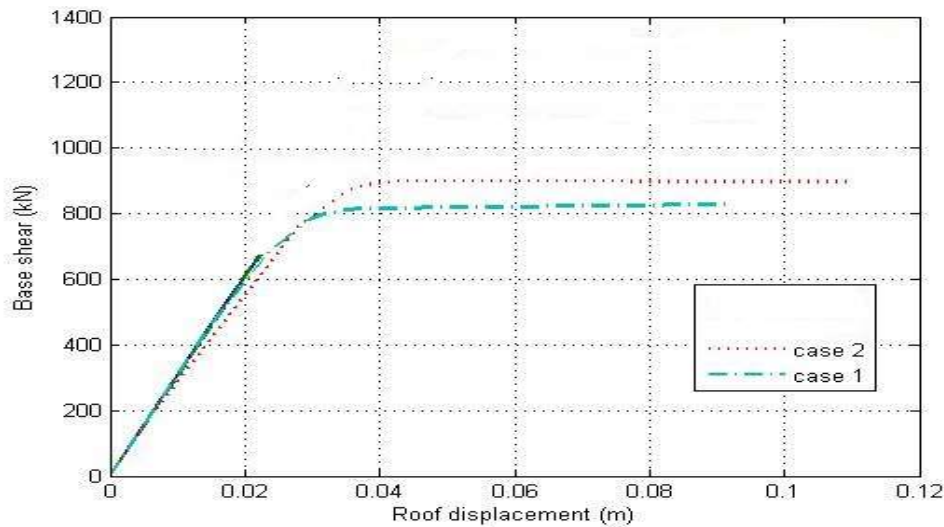
Fig. 3 Demand, Capacity curves in ADRS format and Performance points of buildings
