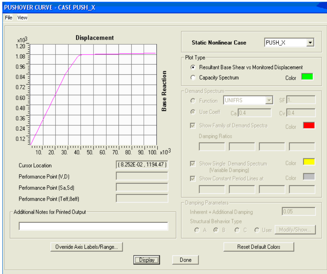
Fig-7 Capacity Curve
