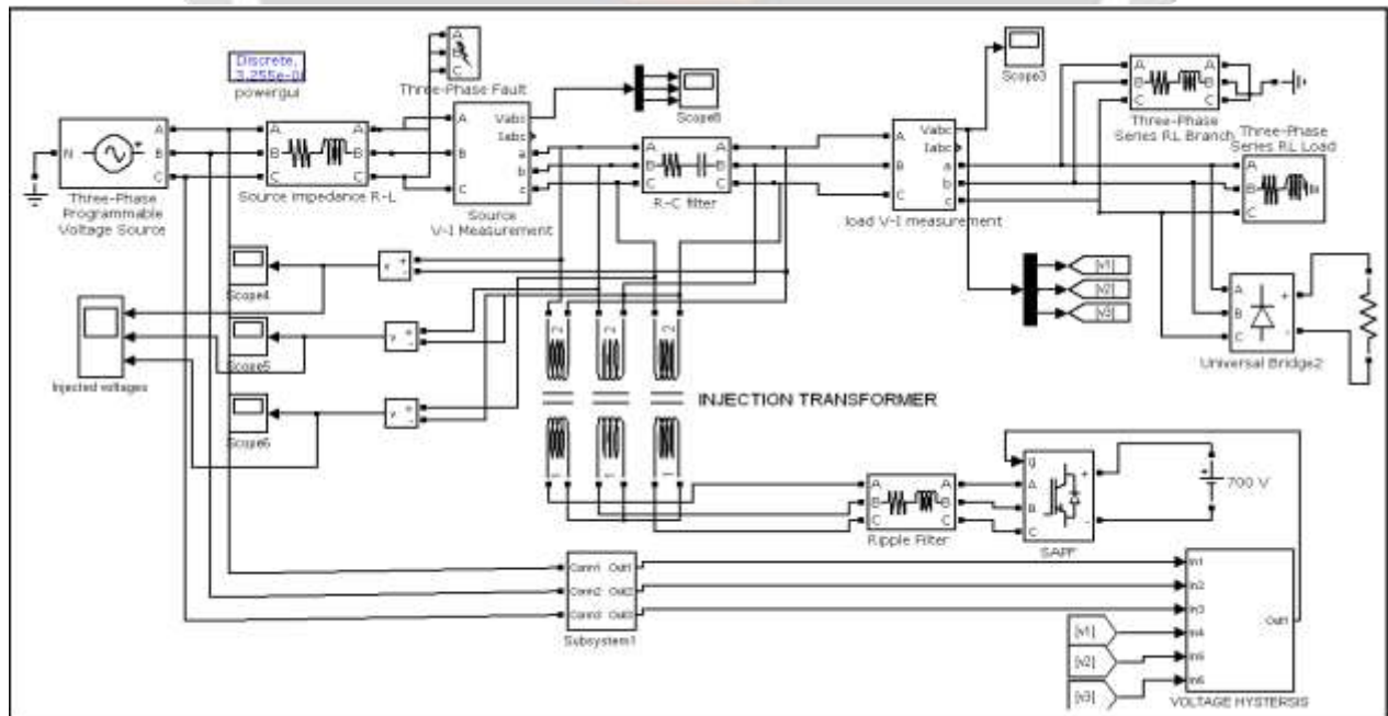
Fig -1: MATLAB simulation model of proposed series active power filter
