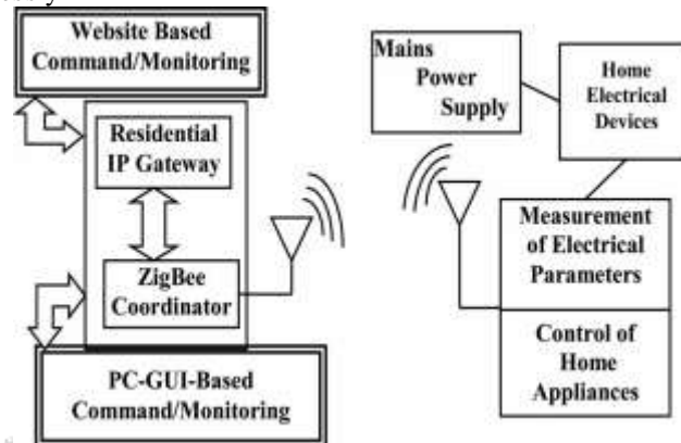
Fig. 1. Functional block diagram of the system.
