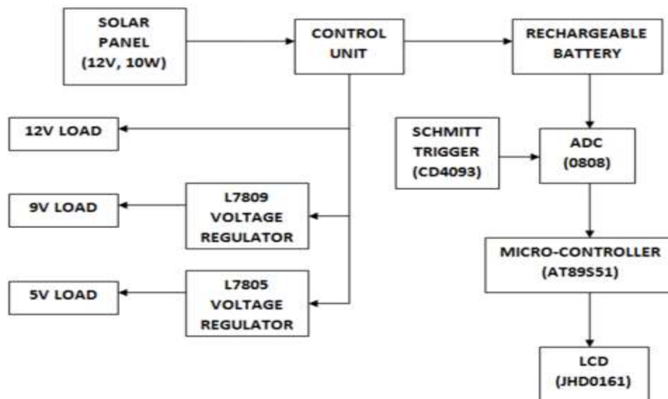
Fig .Block Diagram 1
