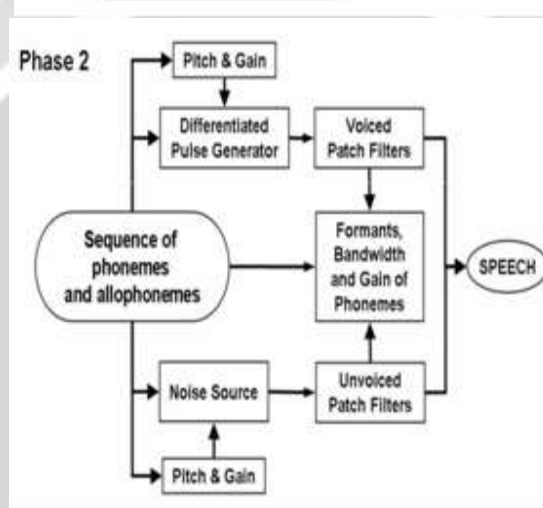
Fig 3: Phases of speech synthesizer
