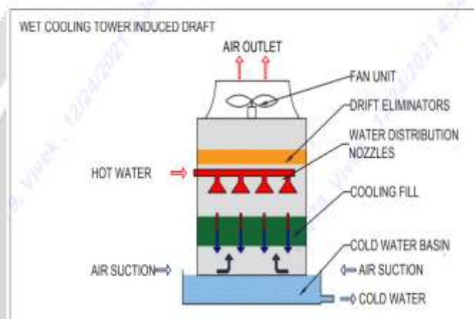
Fig -2: Induced Draft Cooling Tower.
