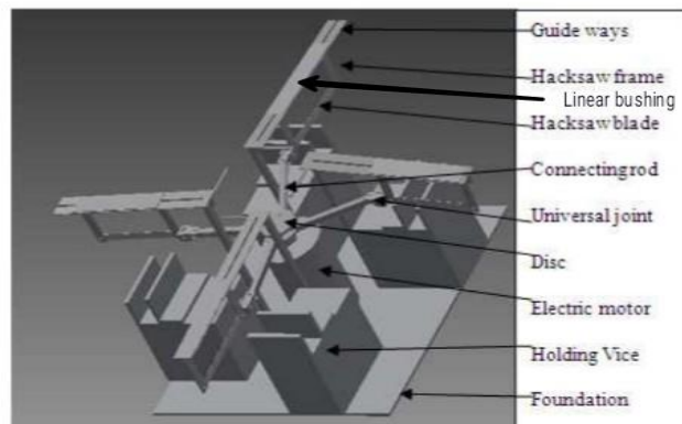
Fig.1 Proposed model of Multi-way power hacksaw machine
