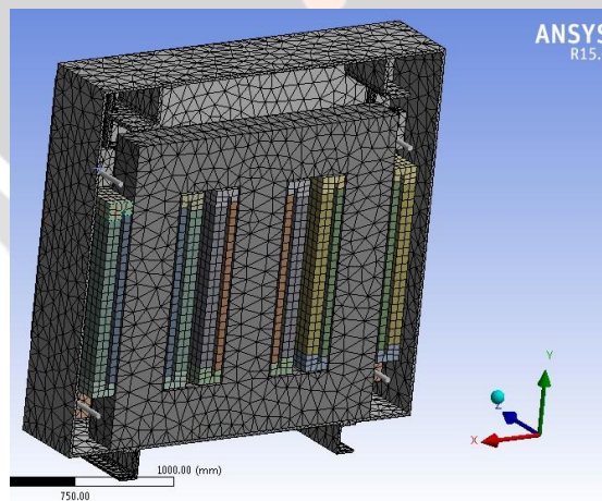
Fig. 2: The grid generated for the selected distribution transformer
