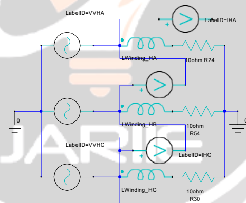
Fig. 4: The electrical model of the given transformer
