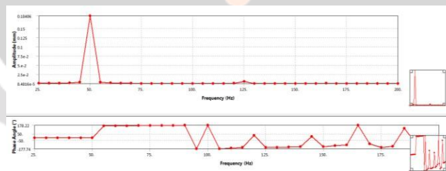
Fig. 10: The frequency characteristic of the shelter's movement in the z direction
