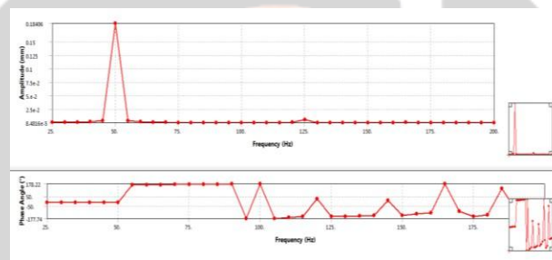
Fig. 9: The frequency characteristic of the shelter's movement in the y direction
