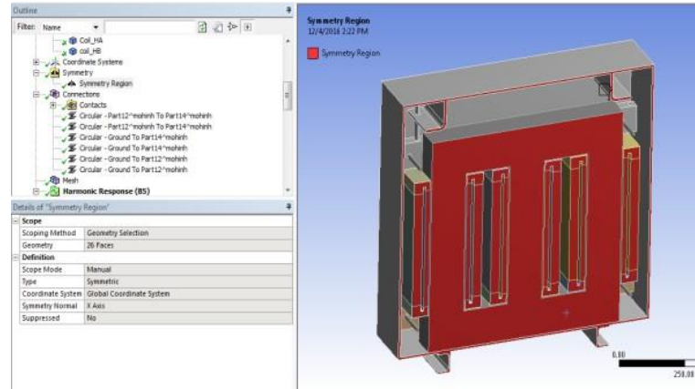
Fig. 3. Setting the symmetrical conditions for the simulation
