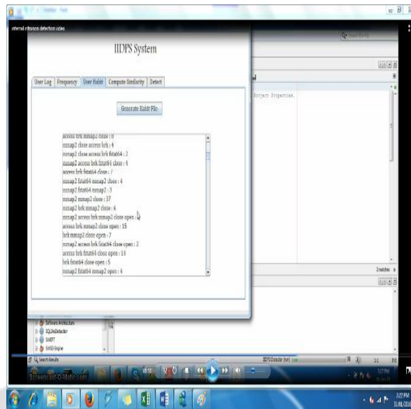
Fig.4 Generate Habit File
