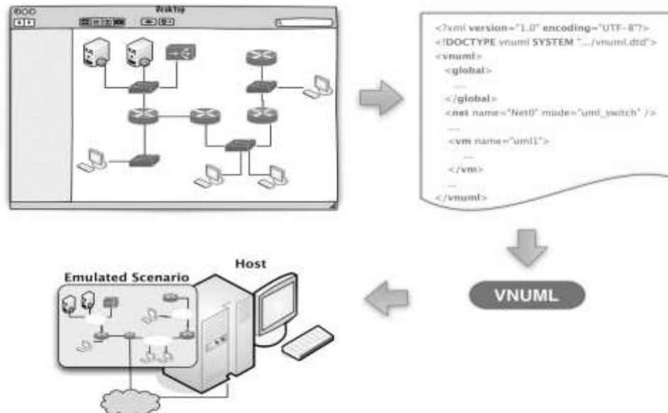
Fig. 1. VNUML development phases
