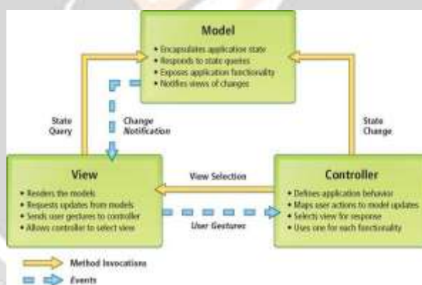
Fig. 2: DFD of MVC
